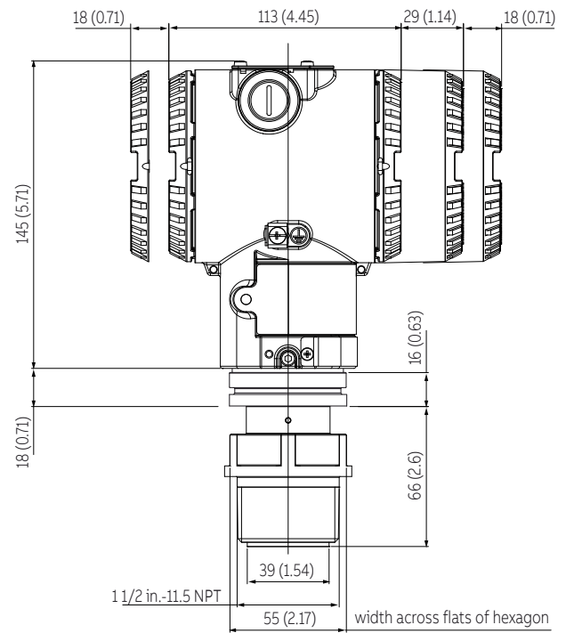
Figure 34 266HRH / 266NRH with barrel housing and direct mount seal S26KN pulp and paper 1 1/2 in. NPT threaded connections
