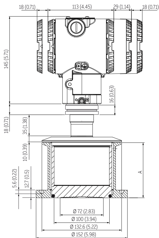
Figure 30 266HRH / 266NRH with barrel housing and direct mount seal S26SS Sanitary extended
