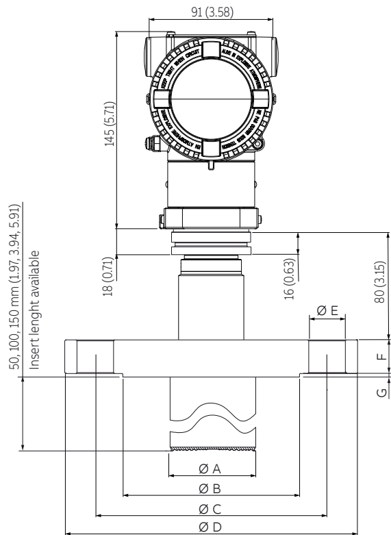
Figure 15 266HRH/266NRH with barrel housing and direct mount seal S26FA/S26FE fixed flange Raised Face ASME and EN 1092/1 smooth and Form B1; S26FE Form E (extension not available). (For dimensions of S26 seals refer to the S26 datasheet)
