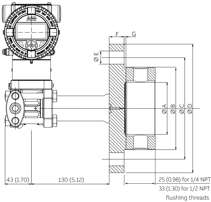
Figure 13 266DRH with barrel housing and direct mount seal S26FA/S26FE fixed flange Raised Face flush diaphragm ASME and EN 1092/1 smooth and Form B1 (flushing ring as option, only for flush version); Form E (For dimensions of S26 seals refer to the S26 datasheet)
