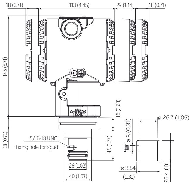
Figure 36 266HRH / 266NRH with barrel housing and direct mount seal S26KN pulp and paper 1 in. sealing with gasket
