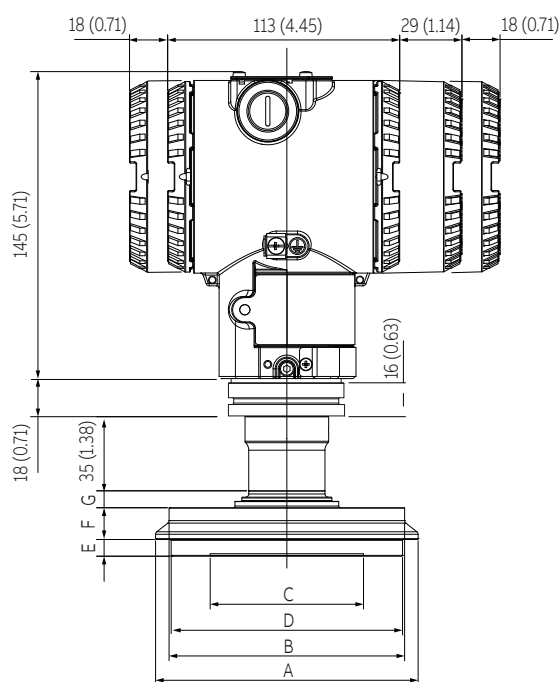
Figure 26 266HRH / 266NRH with barrel housing and direct mount seal S26SS Cherry Burrell (For dimensions of S26 seals refer to the S26 datasheet)
