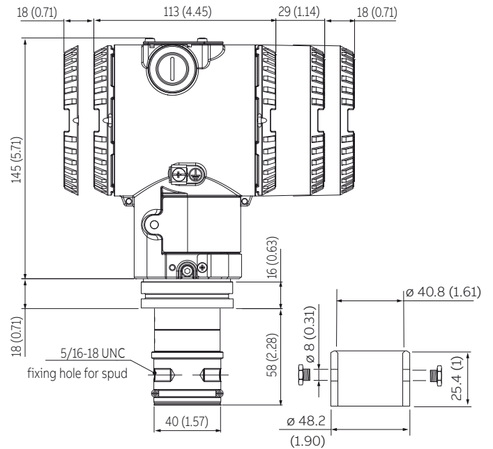
Figure 38 266HRH / 266NRH with barrel housing and direct mount seal S26KN pulp and paper 1 1/2 in. sealing with gasket
