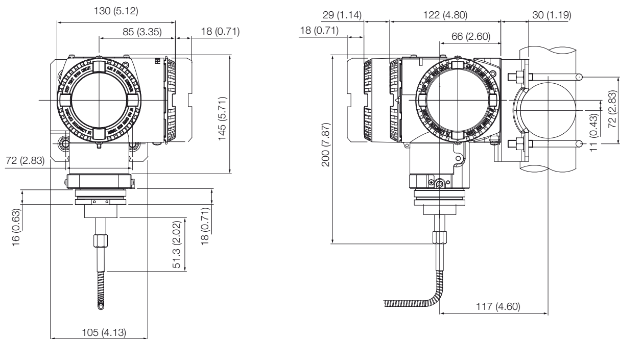
Figure 6 266HRH, 266NRH with barrel housing and remote seal(s) on bracket for vertical or horizontal 60 mm. (2 in.) pipe sensors Z
