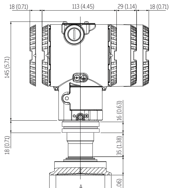
Figure 24 266HRH / 266NRH with barrel housing and direct mount seal S26SS Triclamp (For dimensions of S26 seals refer to the S26 datasheet)
