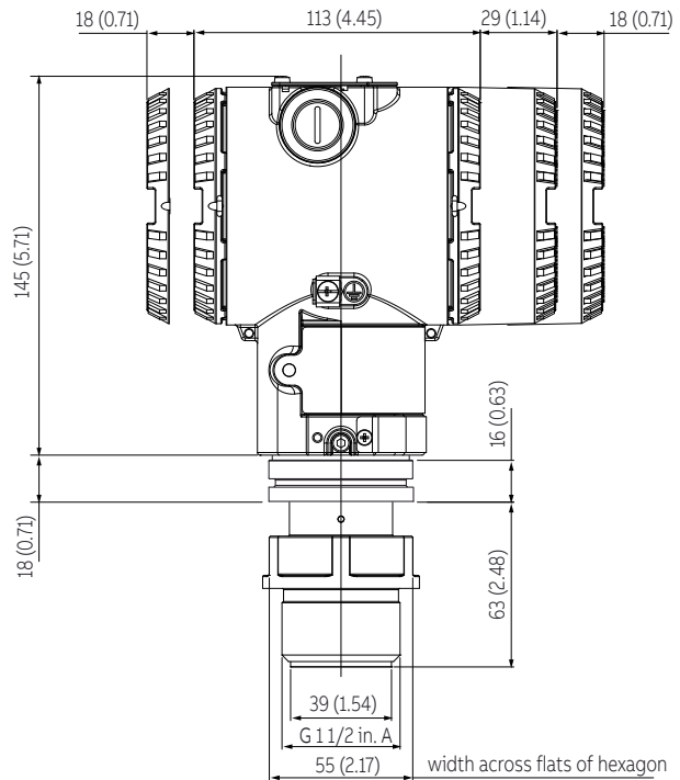
Figure 35 266HRH / 266NRH with barrel housing and direct mount seal S26KN pulp and paper 1 1/2 in. Gas threaded connections
