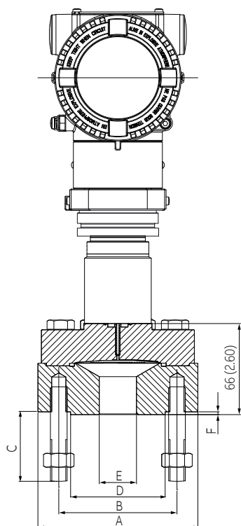
Figure 18 266HRH / 266NRH with barrel housing and direct mount seal S26Mx off-line flanged (For dimensions of S26 seals refer to the S26 datasheet)
