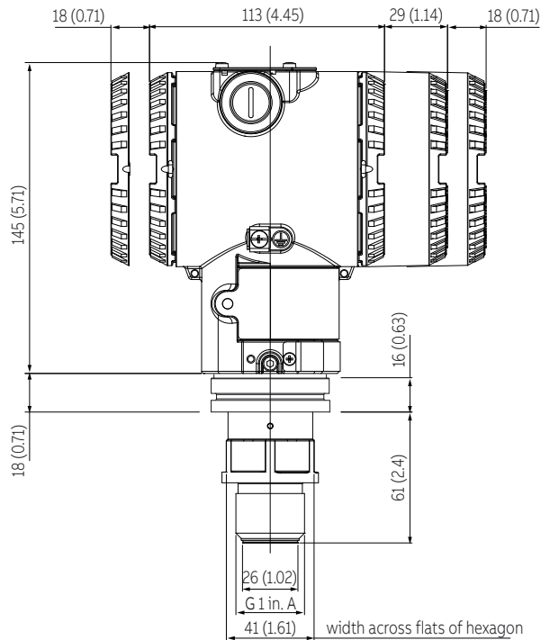
Figure 33 266HRH / 266NRH with barrel housing and direct mount seal S26KN pulp and paper 1 in. Gas threaded connections
