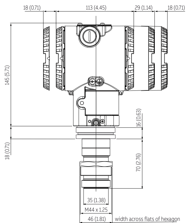
Figure 39 266HRH / 266NRH with barrel housing and direct mount seal S26KN pulp and paper to threaded spud
