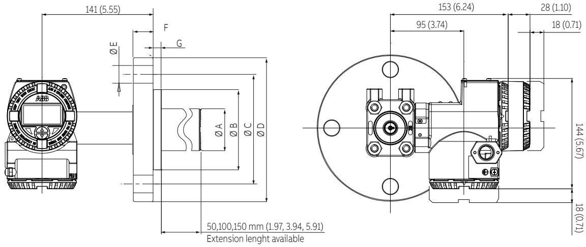
Figure 9 266DRH with DIN housing and direct mount seal S26RA/S26RE/S26RJ rotating flange Raised Face extended diaphragm (For dimensions of S26 seals refer to the S26 datasheet)
