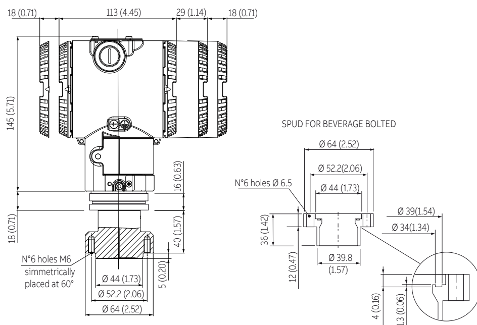
Figure 31 266HRH / 266NRH with barrel housing and direct mount seal S26SS beverage bolted
