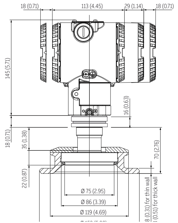
Figure 28 266HRH / 266NRH with barrel housing and direct mount seal S26SS Sanitary flush (For dimensions of S26 seals refer to the S26 datasheet)
