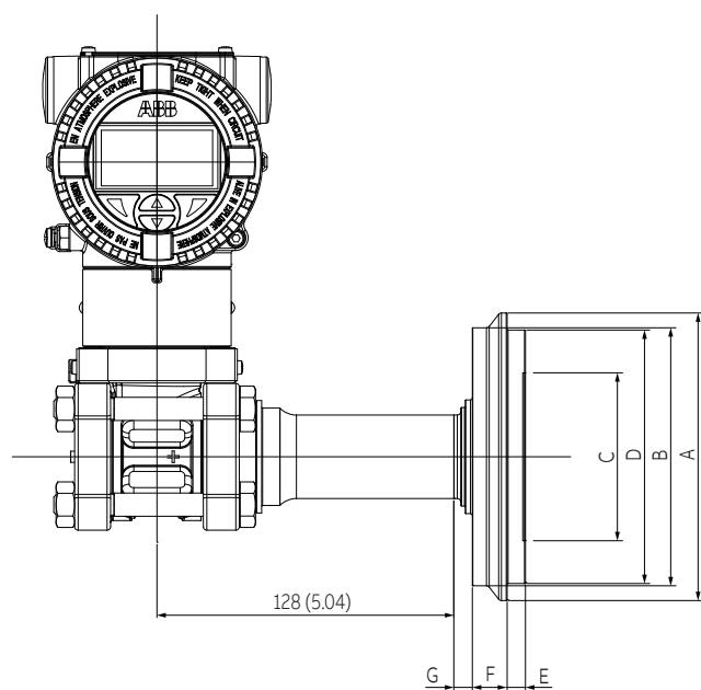
Figure 25 266DRH with barrel housing and direct mount seal S26SS Cherry Burrell (For dimensions of S26 seals refer to the S26 datasheet)
