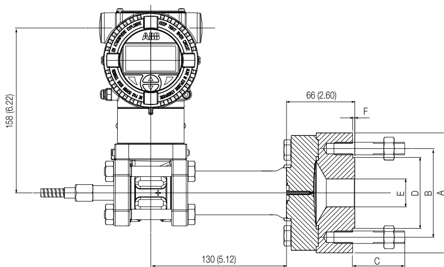
Figure 17 266DRH with barrel housing and direct mount seal S26Mx off-line flanged (For dimensions of S26 seals refer to the S26 datasheet)
