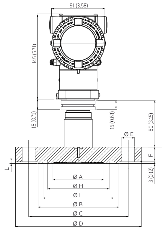
Figure 16 266HRH/266NRH with barrel housing and direct mount seal S26FE fixed flange Raised Face EN 1092/1 Form D (For dimensions of S26 seals refer to the S26 datasheet)
