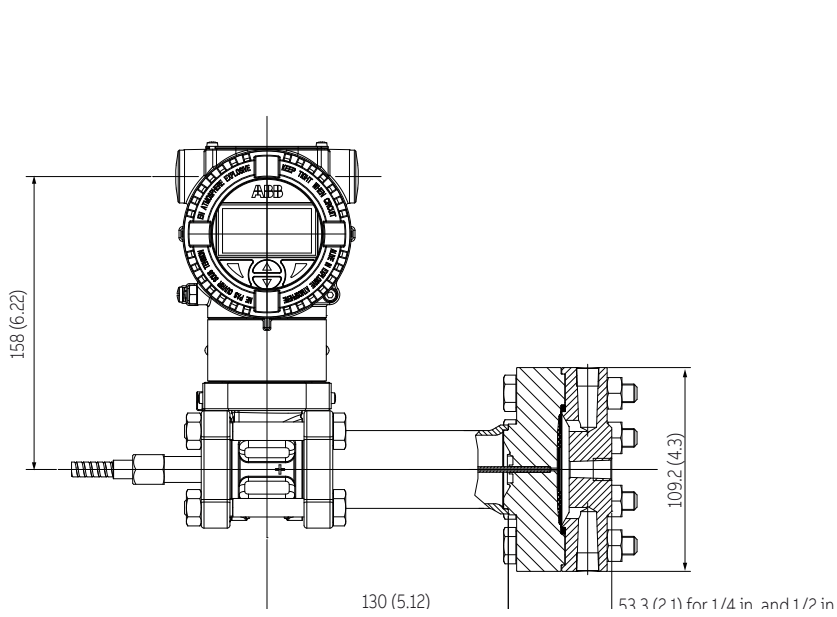
Figure 19 266DRH with barrel housing and direct mount seal S26TT off-line threaded flange
