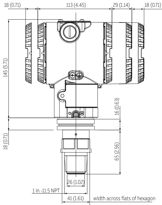
Figure 32 266HRH / 266NRH with barrel housing and direct mount seal S26KN pulp and paper 1 in. NPT threaded connections
