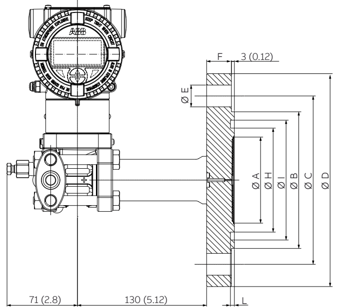
Figure 14 266DRH with barrel housing and direct mount seal S26FE fixed flange Raised Face flush diaphragm EN 1092/1 Form D (For dimensions of S26 seals refer to the S26 datasheet)
