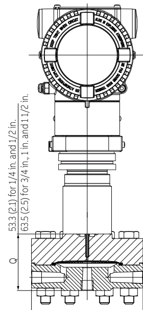
Figure 20 266HRH / 266NRH with barrel housing and direct mount seal S26TT off-line threaded flange
