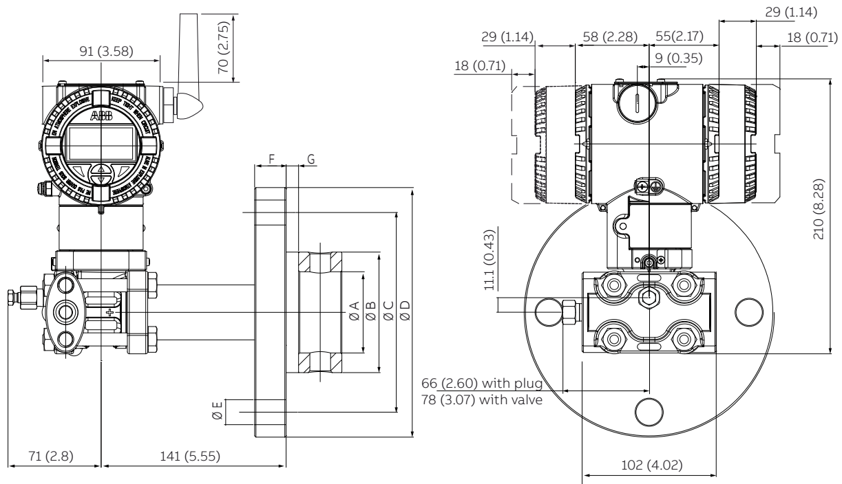
Figure 8 266DRH with barrel housing and direct mount seal S26RA/S26RE/S26RJ rotating flange Raised Face flush diaphragm (For dimensions of S26 seals refer to the S26 datasheet)
