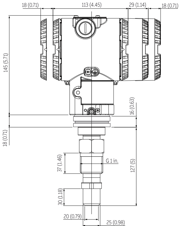
Figure 37 266HRH / 266NRH with barrel housing and direct mount seal S26KN pulp and paper ball valve connections
