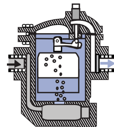
Trap Closes
