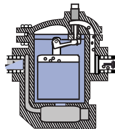
Trap Discharges
