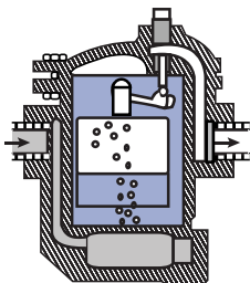
Trap Closed
