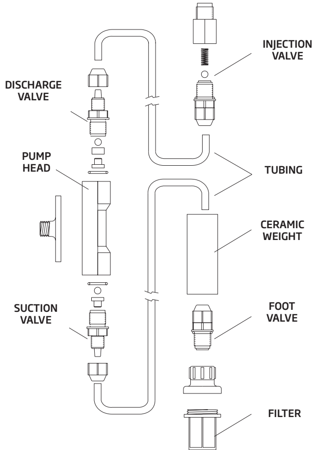
Assembly Diagram
