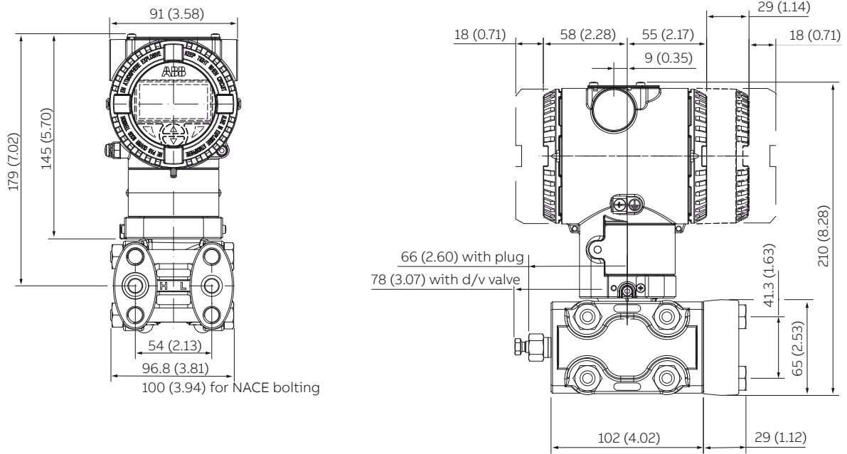
Figure 2 High static transmitter with barrel housing - horizontal flanges
