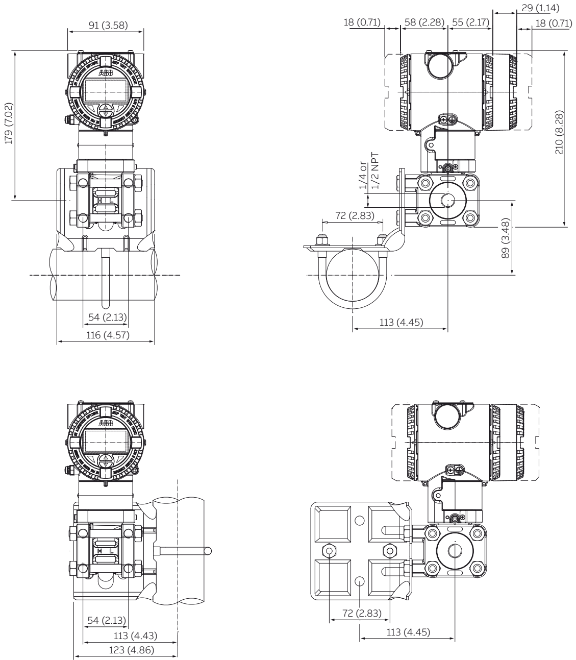
Figure 5 Transmitter with Kynar flanges on bracket for vertical or horizontal 60 mm. (2 in.) pipe mounting
