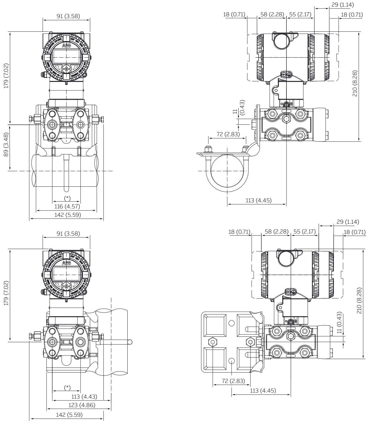
Figure 4 Transmitter on bracket for vertical or horizontal 60 mm. (2 in.) pipe mounting
